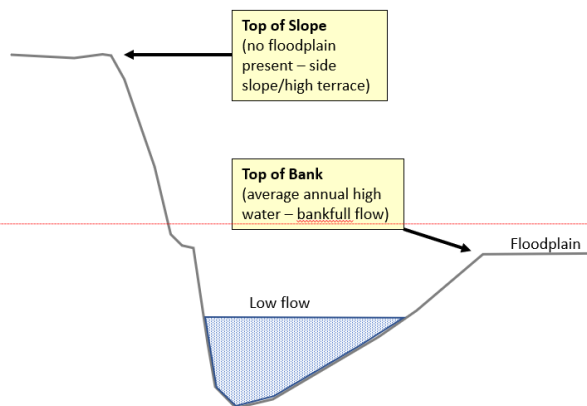
Figure 5-4 Diagram showing the Top of Bank where stream flows onto a floodplain and Top of Slope where floodplain access is not present.
