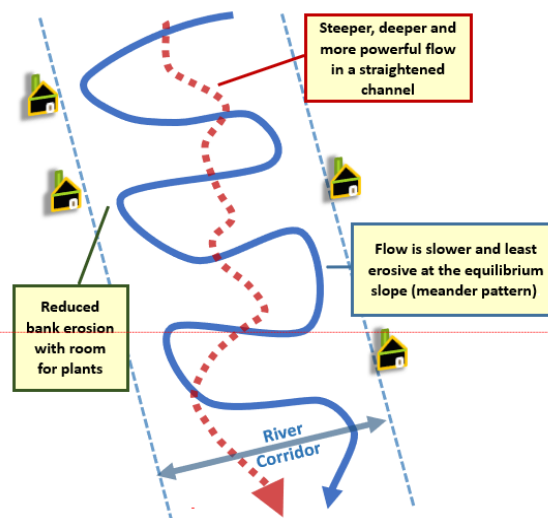
Figure 34-River Corridor Diagram showing room for river channel adjustments to minimize slope and erosive power.
