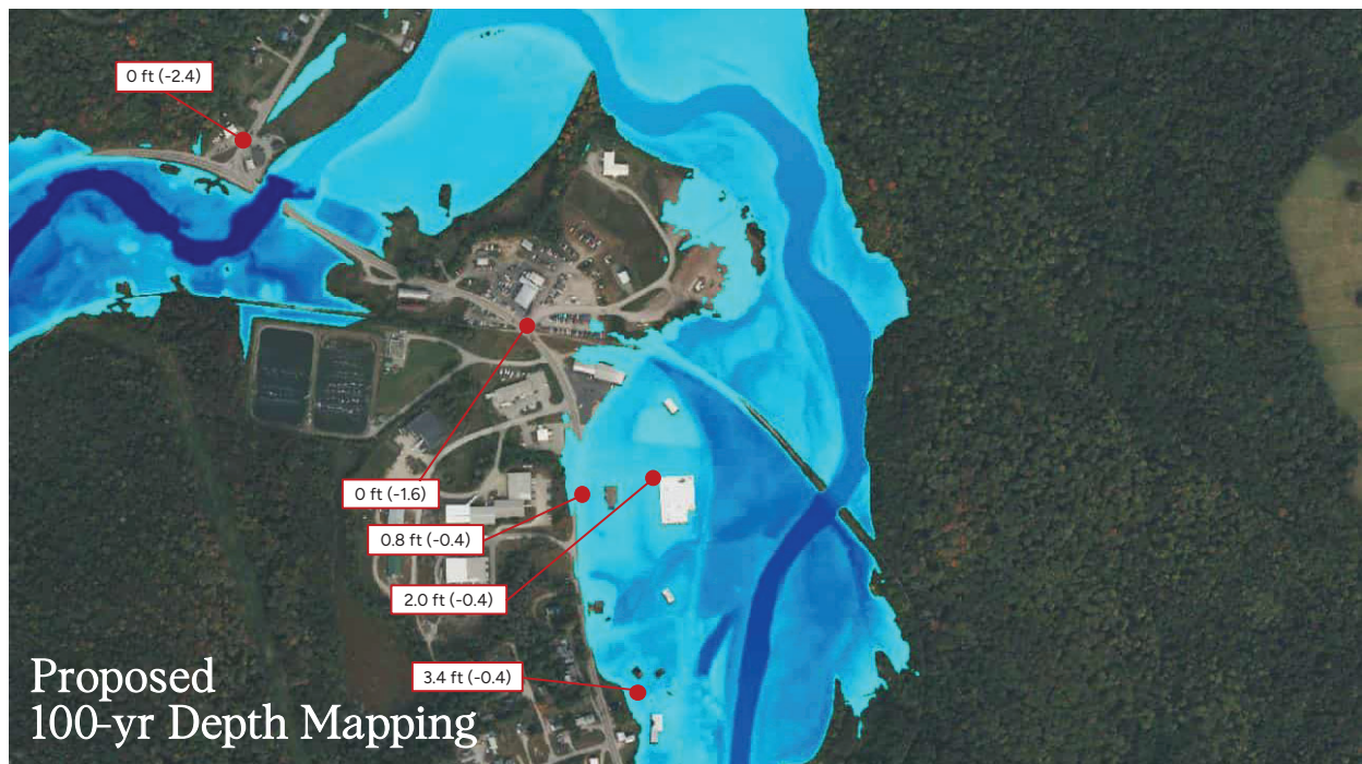
Figure 46: Depth mapping of proposed dam removal for a large flood
