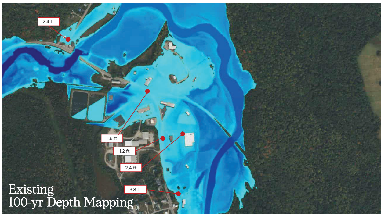
Figure 45: Depth mapping of existing conditions for a large flood
